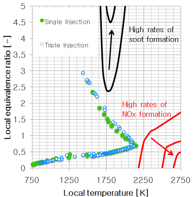
In this diagram, the mixture temperature and equivalence ratio are plotted at peak pressures for both cycles. The regimes of high rates of soot and NO x formation are also presented. The marks in blue and green represent the local compositional state of the in-cylinder mixture, demonstrating the degree of mixture stratification in terms of both equivalence ratio and temperature. All regions of the combustion chamber avoided those regimes of excessive formation rate of soot and NO x .
